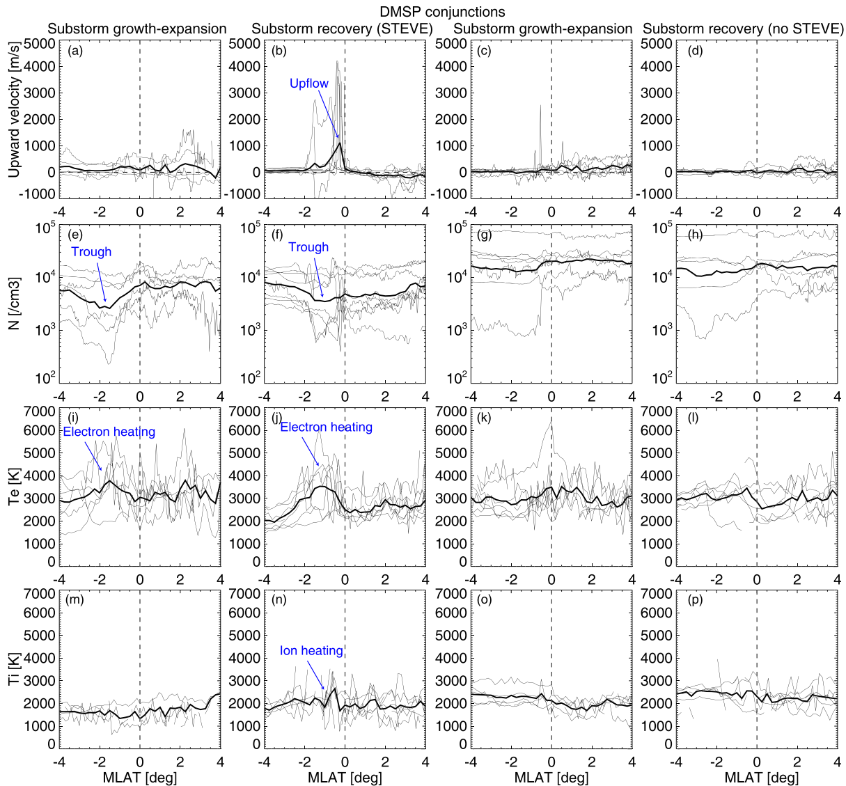
Figure 8. Same as Figure 7 except that the panels shown are (a–d) upward velocity, (e–h) ion density, (i–l) electron temperature, and (m–p) ion temperature.
